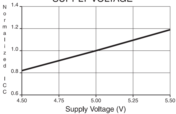
NORMALISED SUPPLY CURRENT vs. SUPPLY VOLTAGE
