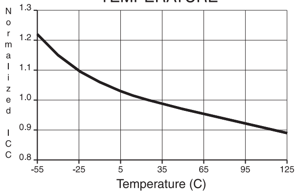
NORMALISED SUPPLY CURRENT vs. TEMPERATURE
